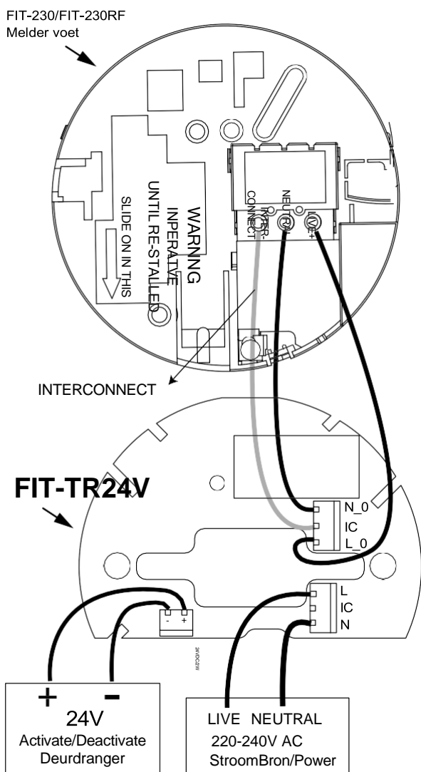
Fig.1. Installation Instruction (connect with 1pcs smoke alarm)
