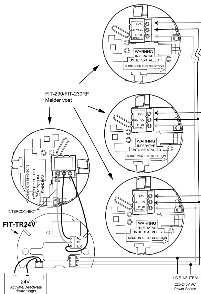
Fig.2. Installation instruction (more than 1pcs smoke alarm)
